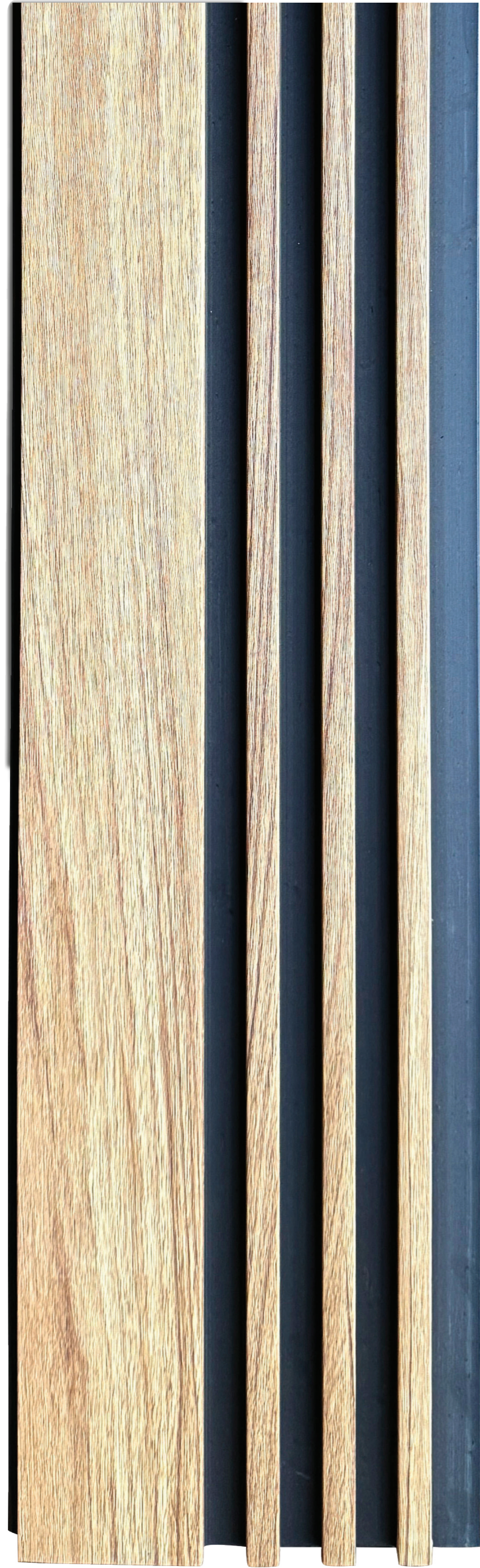
BB 3-PLUS 46 179X16X2900mm
